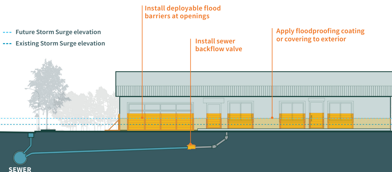
Section 05: Illustrative section of dry floodproofing measures. Drawing not to scale.
