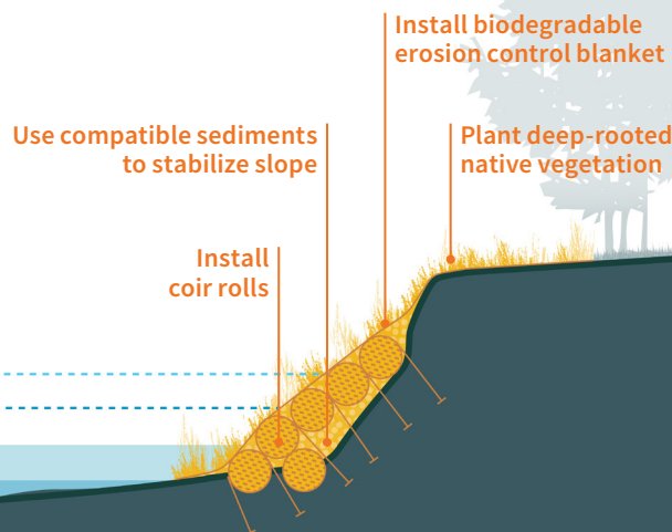
Section 16: Illustrative section of bank stabilization. Drawing not to scale.
