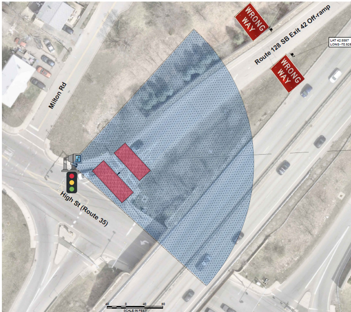
Wrong Way Vehicle Detection System Installation
