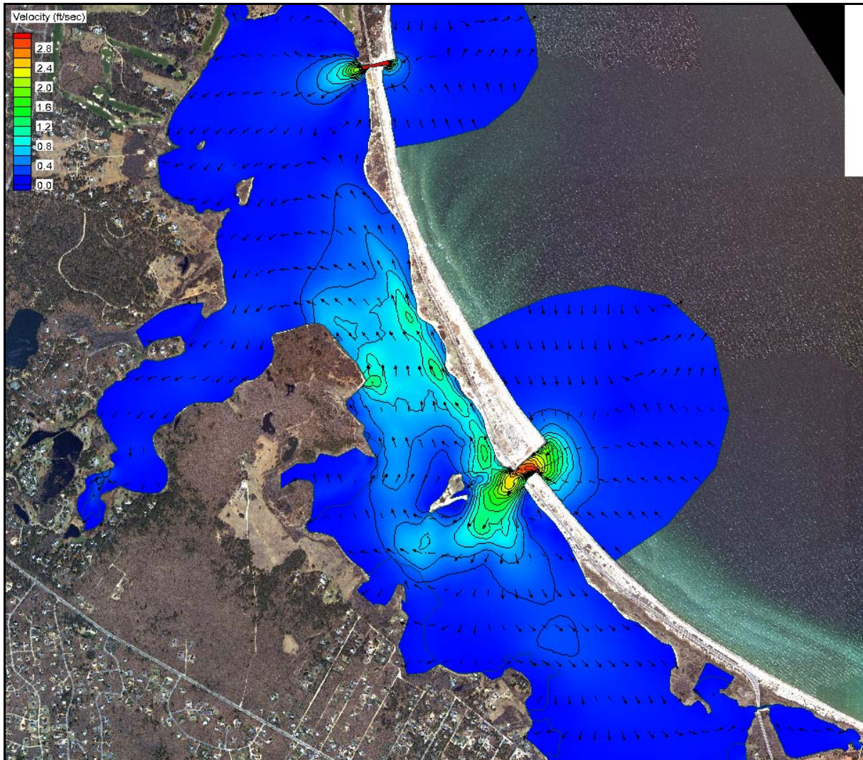
Figure V-20. Example of hydrodynamic model output in Sengekontacket Pond for a single time step where maximum flood velocities occur for this tide cycle. Color contours indicate flow velocity, and vectors indicate the direction and magnitude of flow.
