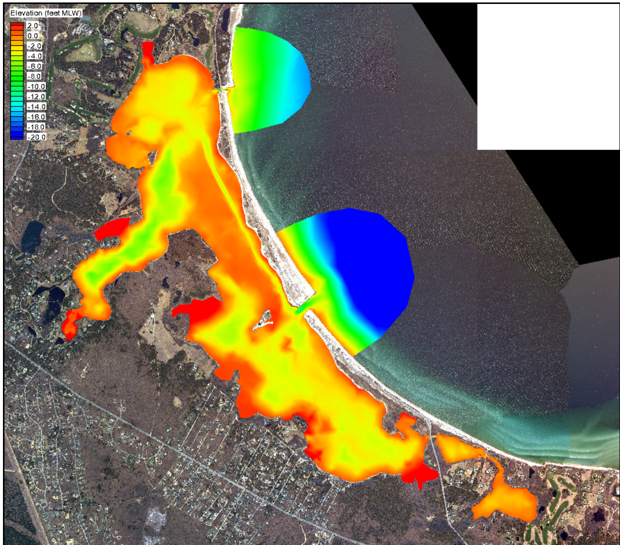
Figure V-9. Depth contours of the completed Sengekontacket Pond finite element mesh.
