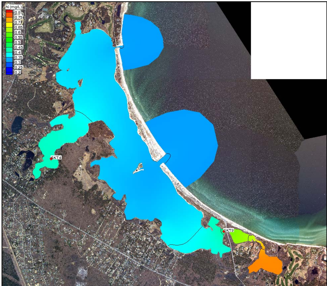
Figure VI-7. Contour plots of modeled total nitrogen concentrations (mg/L) in Sengekontacket Pond System, for projected build-out loading conditions, and bathymetry. The approximate locations of the sentinel threshold stations for Sengekontacket Pond System (SKT-4 and SKT-9) are shown.
