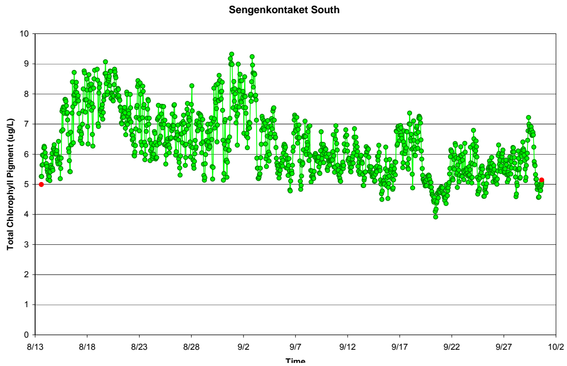
Figure VII-6. Bottom water record of Chlorophyll-a in the Sengekontacket South station, Summer 2004. Calibration samples represented as red dots.
