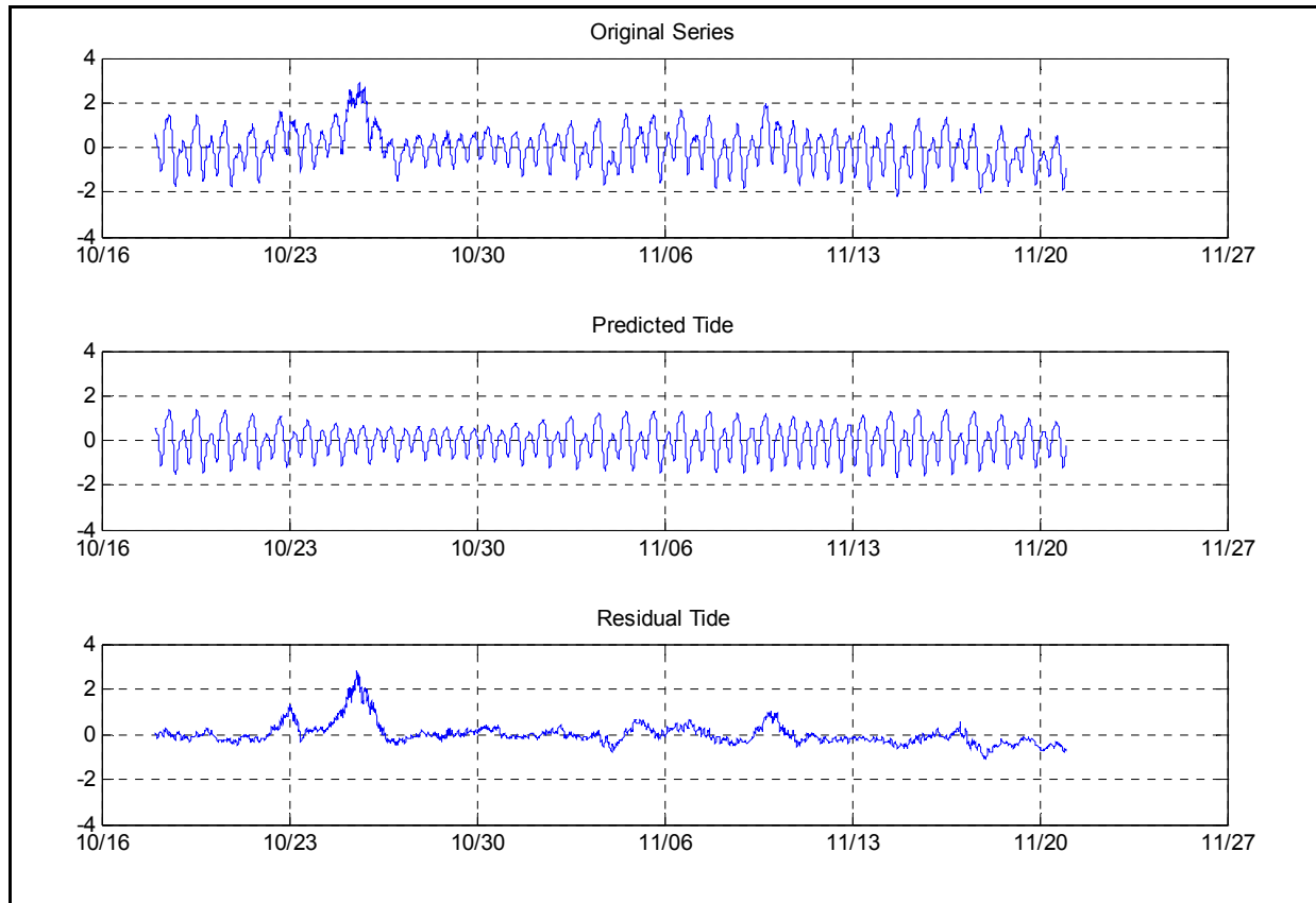
Figure V-7. Results of the harmonic analysis and the separation of the tidal from the non-tidal, or residual, signal measured in Nantucket Sound at gauge location S-1.
