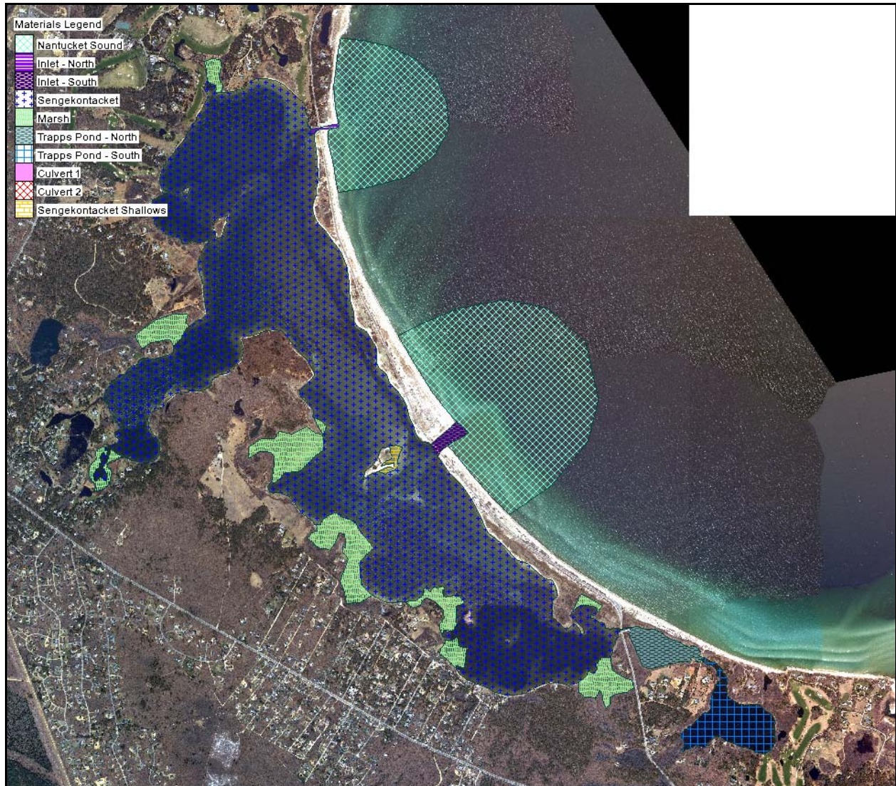
Figure V-8. The model finite element mesh developed for Sengekontacket Pond system. The model seaward boundaries were specified with forcing functions consisting of water elevation measurements obtained in Nantucket Sound.
