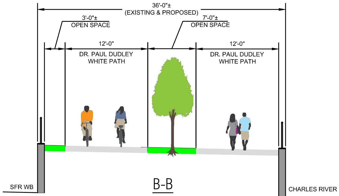
Dr. Paul Dudley White Path Typical Sections (Looking North)
