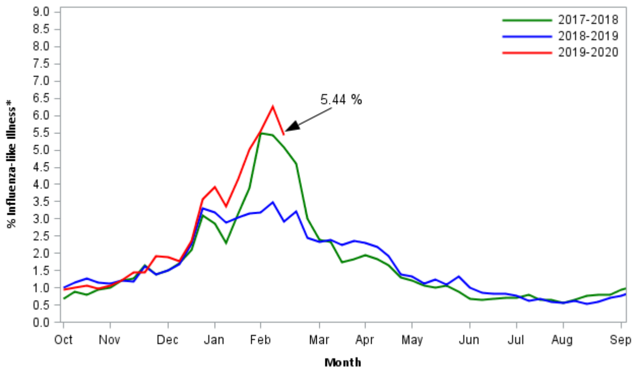
Figure 1: Percentage of ILI visits reported by sentinel provider sites September 29, 2019 – February 15, 2020
