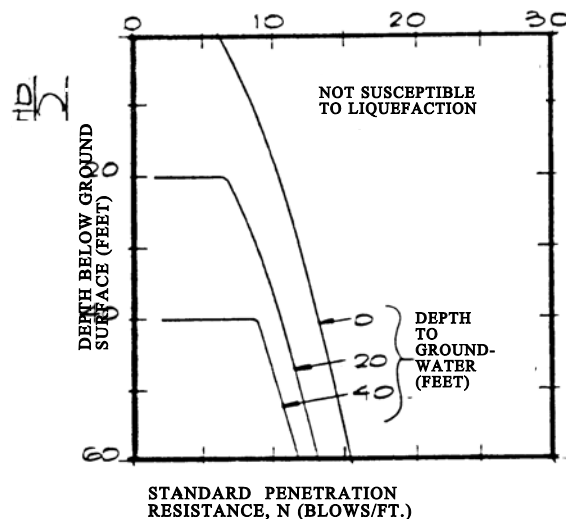
Figure 1805.3 LIQUEFACTION SUSCEPTIBILITY
