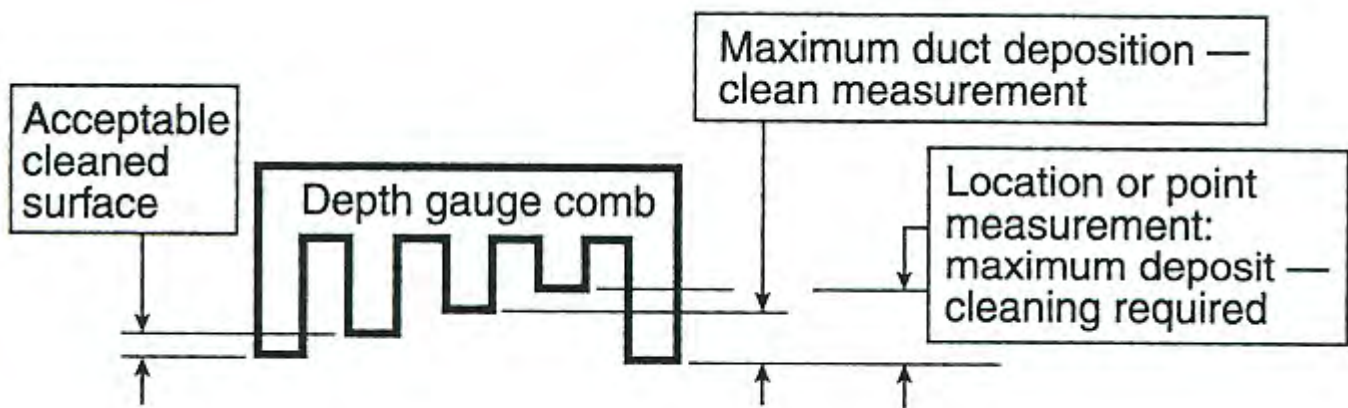
FIGURE A.50.5.6.2 Depth Gauge Comb. [96: Figure A.11.6.2]
