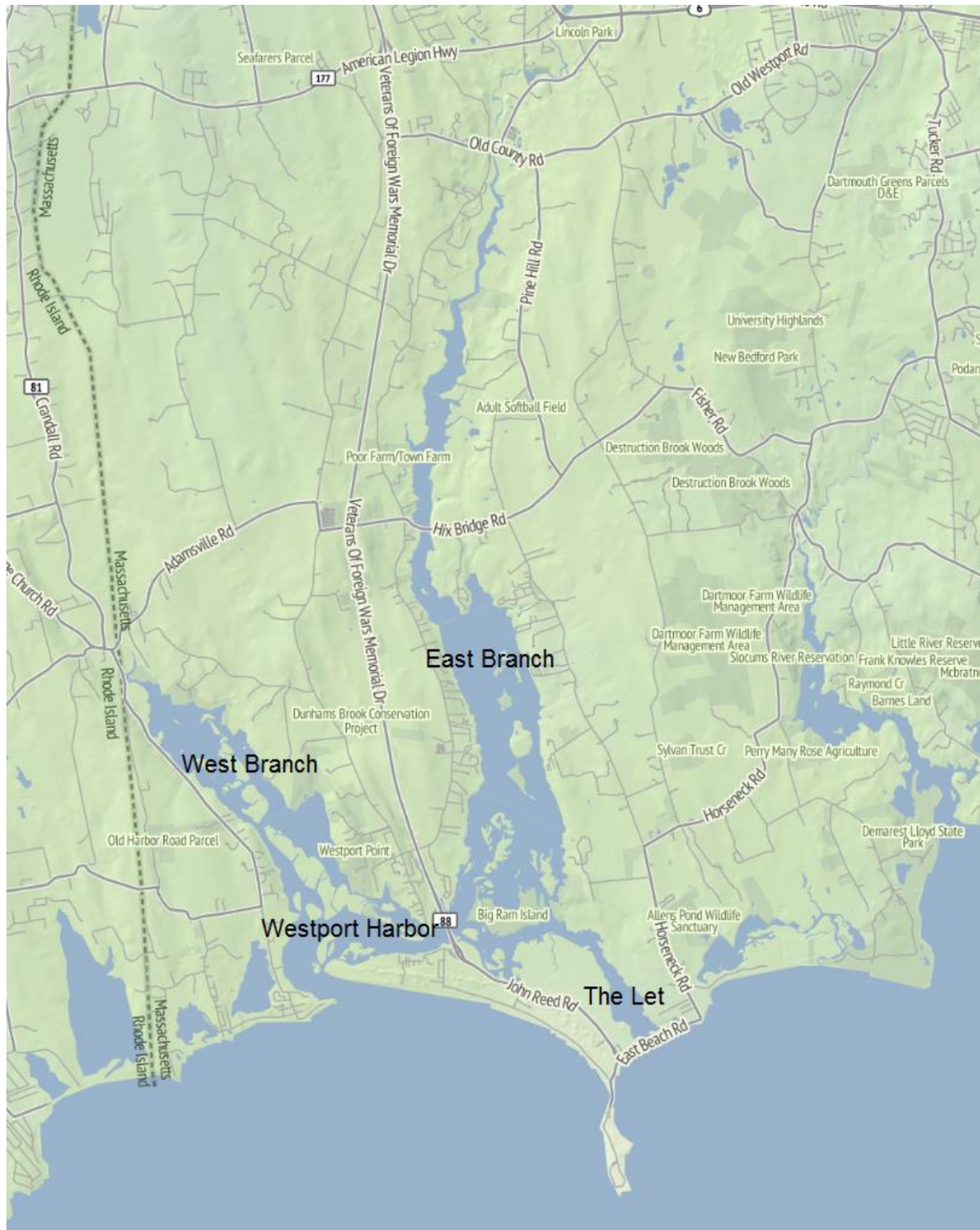
Figure 1: Westport River Embayment System (map made via gmap, courtesy Kahle and H. Wickham 2013)
