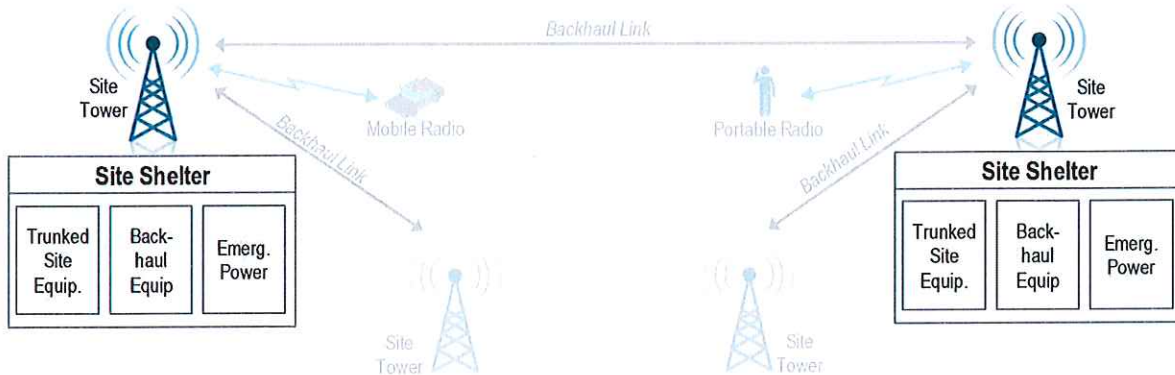
Figure 2-24: Site Equipment
