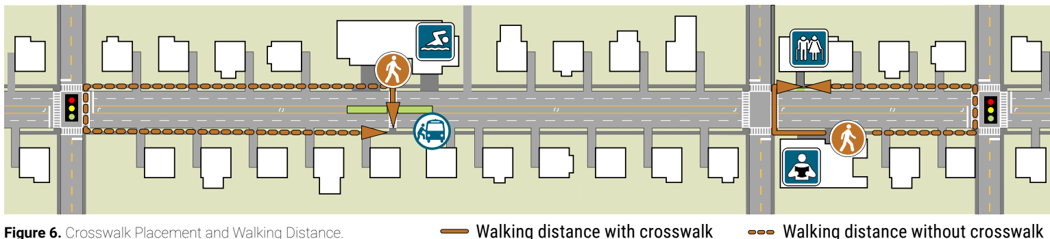
Figure 6. Crosswalk Placement and Walking Distance. Credit: FHWA Achieving Multimodal Networks
