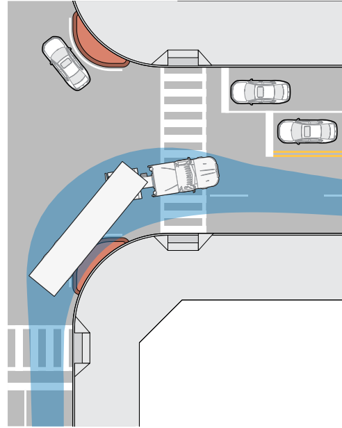
Figure 10. Mountable truck apron
