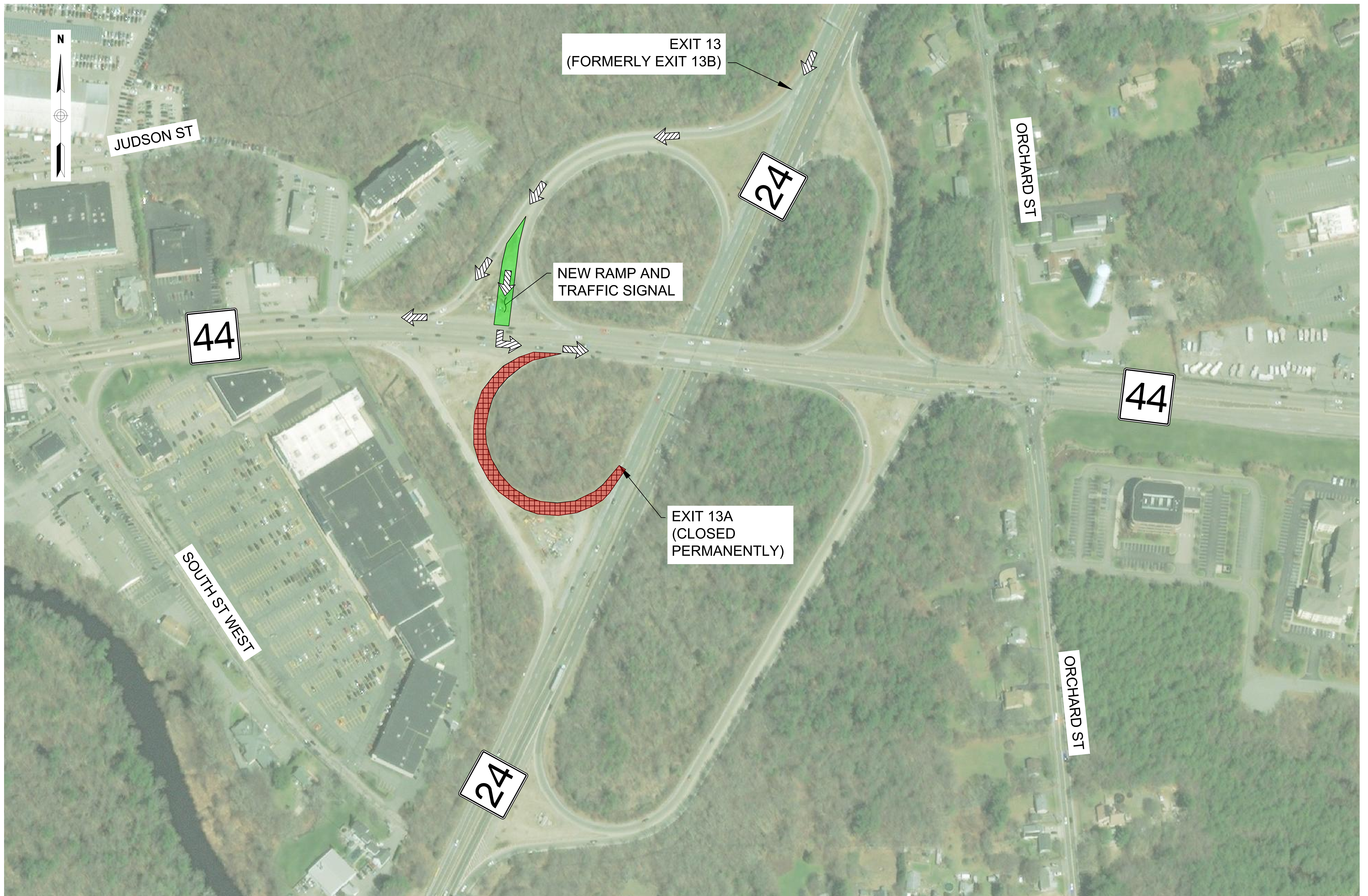
Exit 13 Ramp Re-configuration Graphic
