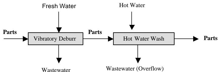
FIGURE 1: FLOW DIAGRAMS - BEFORE
