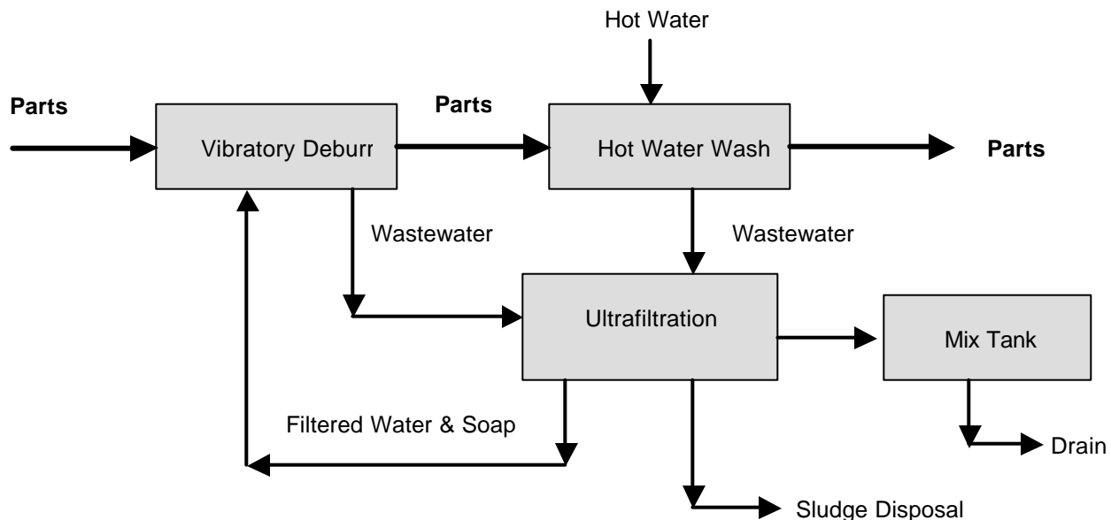
FIGURE 2: FLOW DIAGRAMS - AFTER
